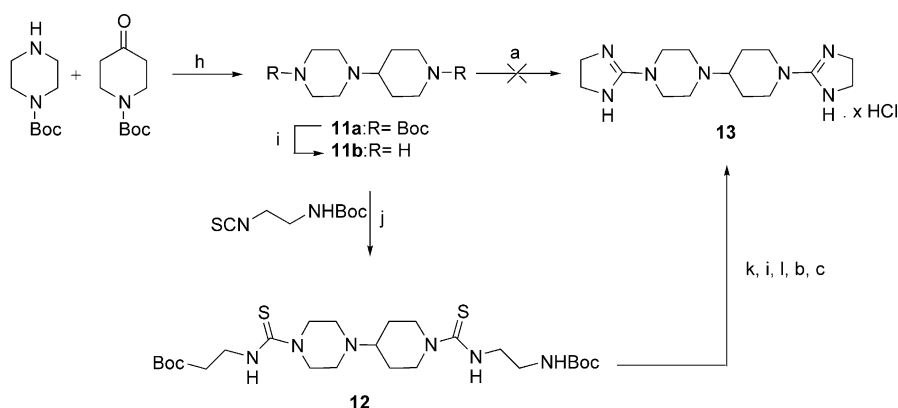
Scheme 4. (h) \text{NaBH}_3\text{CN} , AcOH, MeOH, pH 7 (65%); (i) TFA, \text{CH}_2\text{Cl}_2 ; (j) THF, rt, 2 days, (50%); (k) EtI, EtOH, 60^\circ\text{C} ; (l) NaOEt, EtOH, rt.
