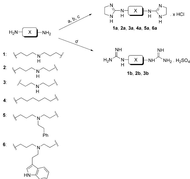
Scheme 1. (a) 2-Methylmercapto-4,5-dihydroimidazole iodide, MeOH, reflux.
