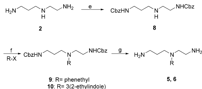
Scheme 3. (e) benzylcyanoformate, \text{CH}_2\text{Cl}_2 (79%); (f) \text{K}_2\text{CO}_3 , \text{CH}_3\text{CN} , reflux; (g) \text{H}_2/\text{Pd/C} 10%, MeOH.
