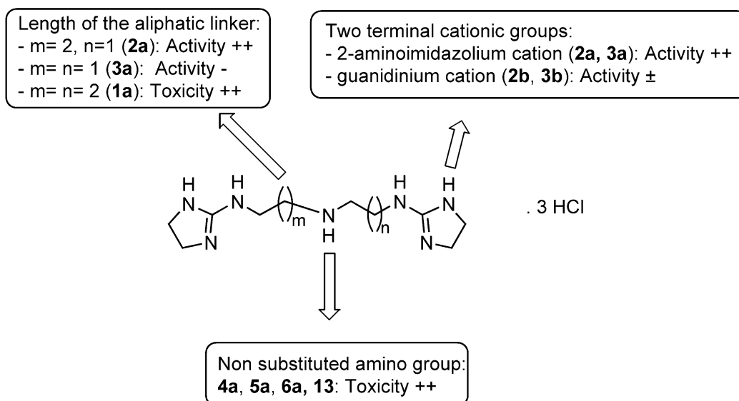
Figure 1. SAR studies on compound 2a .
